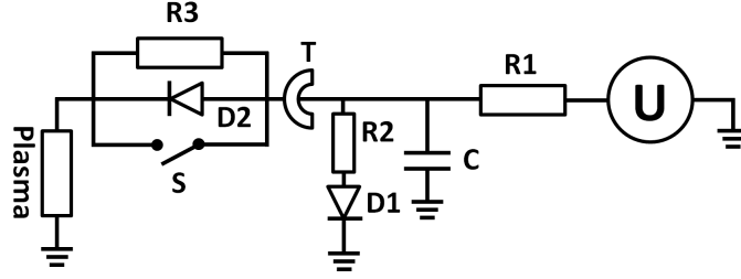
Figure 8.11: Electrical layout of the discharge electronics. Negative polarity of the charging voltage U was used in the final setup.
