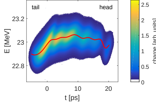
Figure 7.7: Exemplary longitudinal phase space of the triangularly shaped bunches. The red line shows the slice mean energy.
