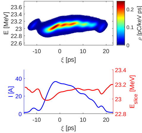
Figure 10.3: Longitudinal phase space of the (677 \pm 70) pC driver & witness beam, measured in the high energy dispersive section HEDA2 [top; no plasma interaction, compare Fig. 10.2 (a)]. Bottom plots show bunch current profile (blue) and slice energies (red).
