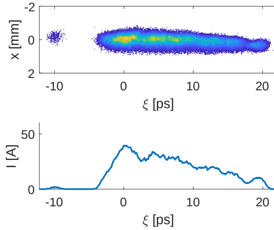
Figure 10.6: Transverse-longitudinal projection in the co-moving frame \xi = z/c - t for the 518 \pm 16 pC driver/witness beam that was measured to drive a PWFA with a transformer ratio of 4.6^{+2.2}_{-0.7} .
