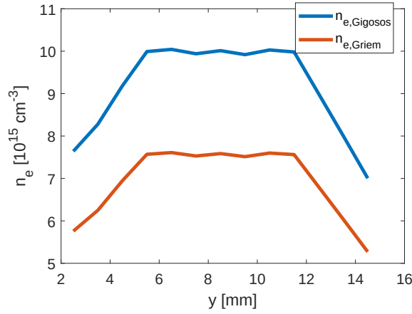
Figure 8.20: Plasma densities for different vertical positions of the spectrometer fiber. Measurements were taken with a 3 \mu\text{s} delay to the discharge current pulse.
