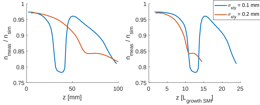
Figure 8.25: Evolution of simulated measured plasma density n_{meas} relative to the actually simulated density n_{sim} of 0.5 \times 10^{15} \text{ cm}^{-3} along the plasma for two different probe bunches, with 510 pC, 27 ps FWHM length. The transverse RMS size \sigma_{x/y} of the bunches at the entrance into the plasma was varied and the curves are measured in geometrical distances (left) and SMI growth lengths (right).
