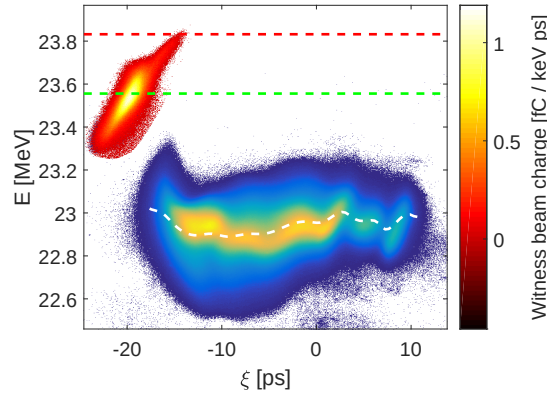
Figure 10.11: LPS measurement of the beam that showed a transformer ratio of 5.0^{+1.5}_{-0.4} with witness charge density colourmap scaled to the maximum measured witness intensity after plasma wakefield interaction [compare Fig. 10.10 (b)].
